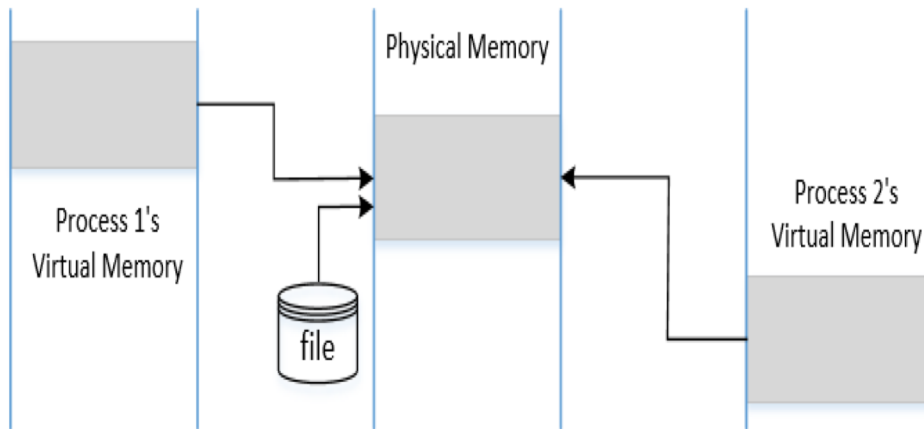
(a) MAP_SHARED
